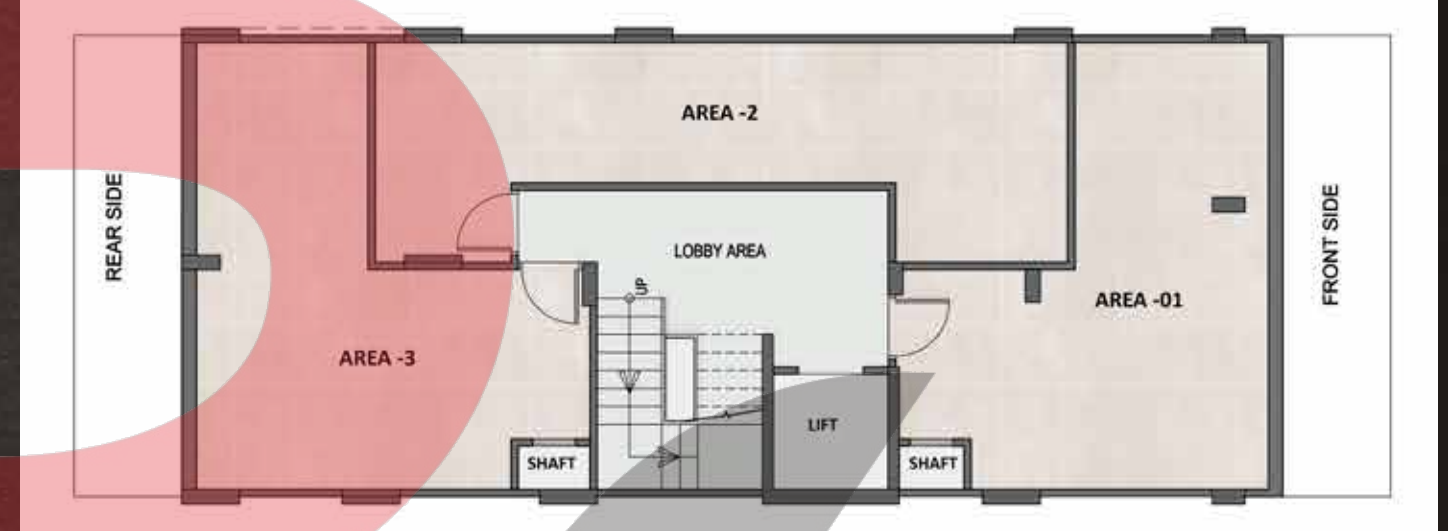
BASEMENT PLAN
