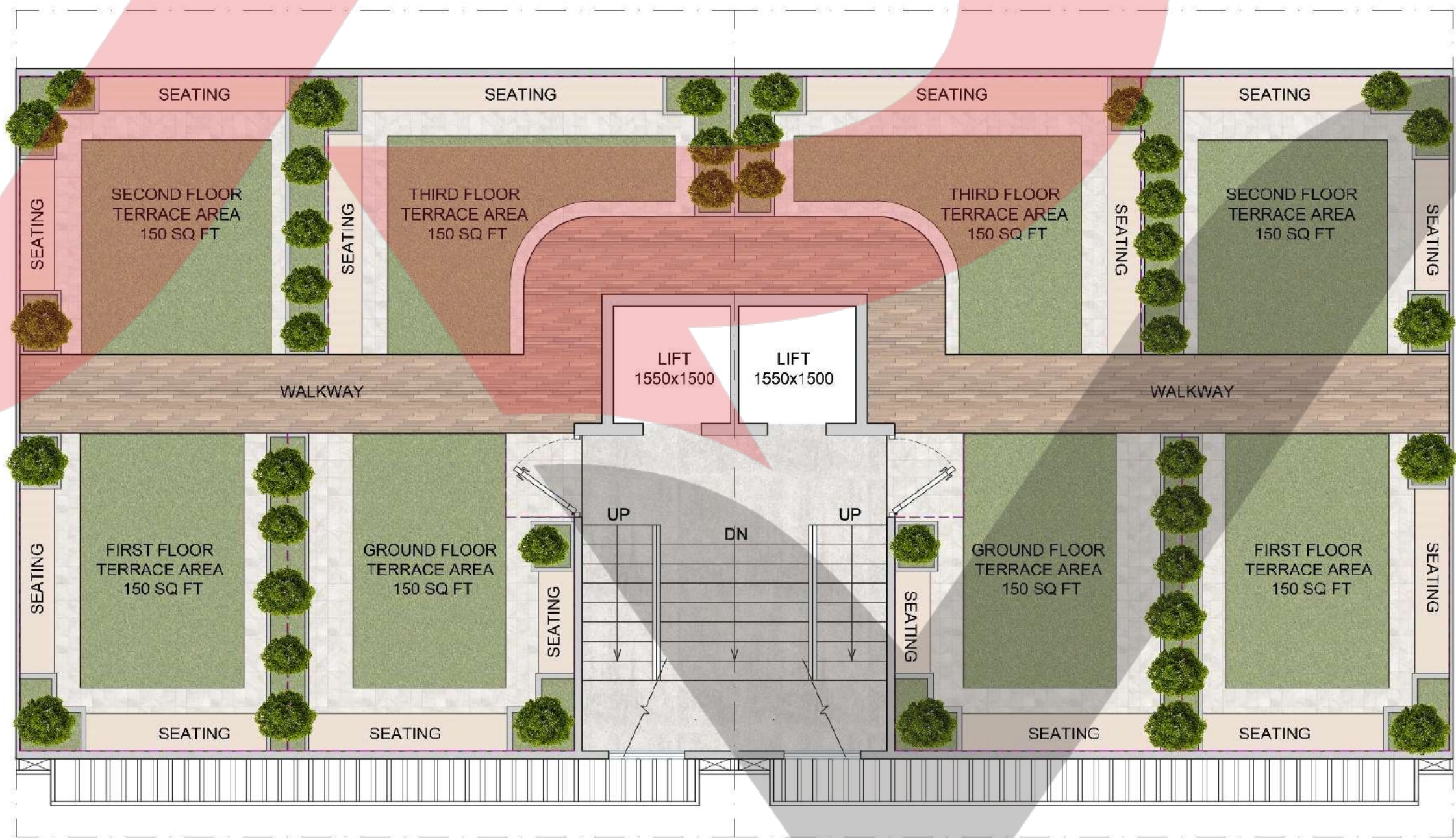
TERRACE PLAN
