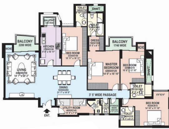
(3000 Sq. Ft.)
