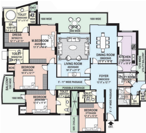
(4098 Sq. Ft.)
