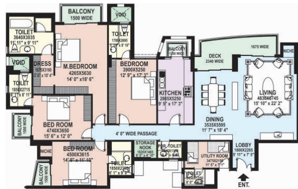
(3430 Sq. Ft.)
