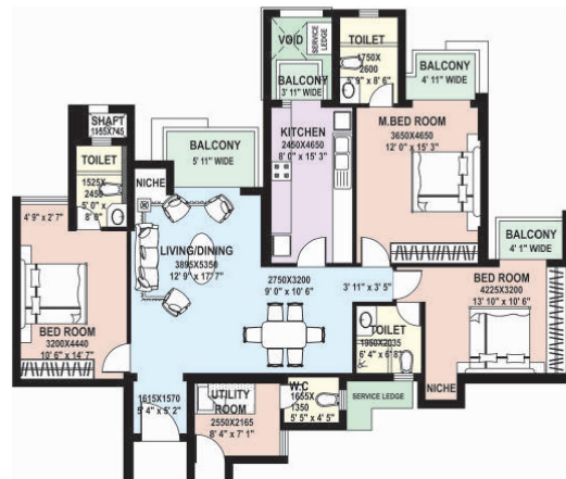
(1975 Sq. Ft.)
